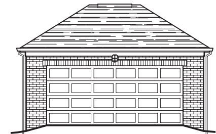
Rear Garage Elevation
